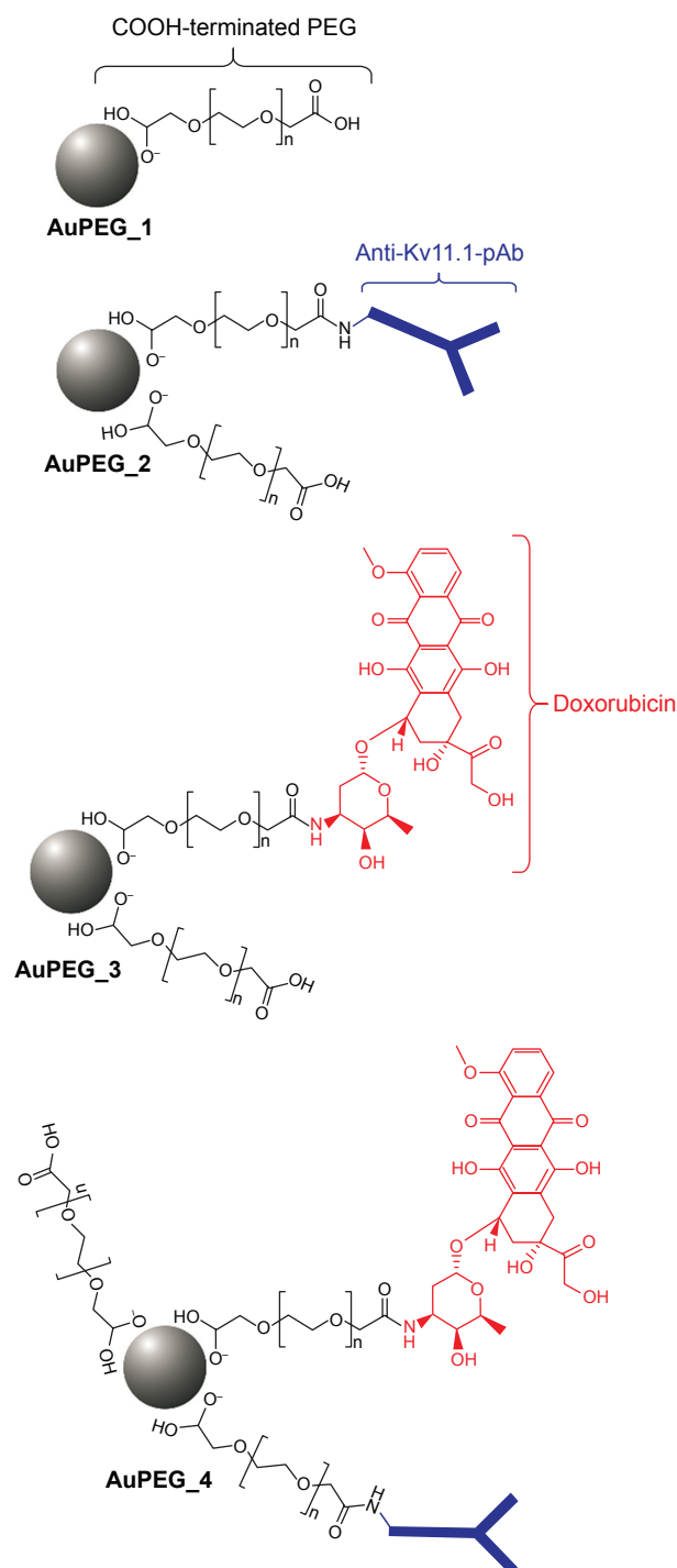
Figure 1 Schematic representation of PEG-AuNPs chemical structures. Note: Drawings are not in scale and are not intended as representative of the full sample composition.
