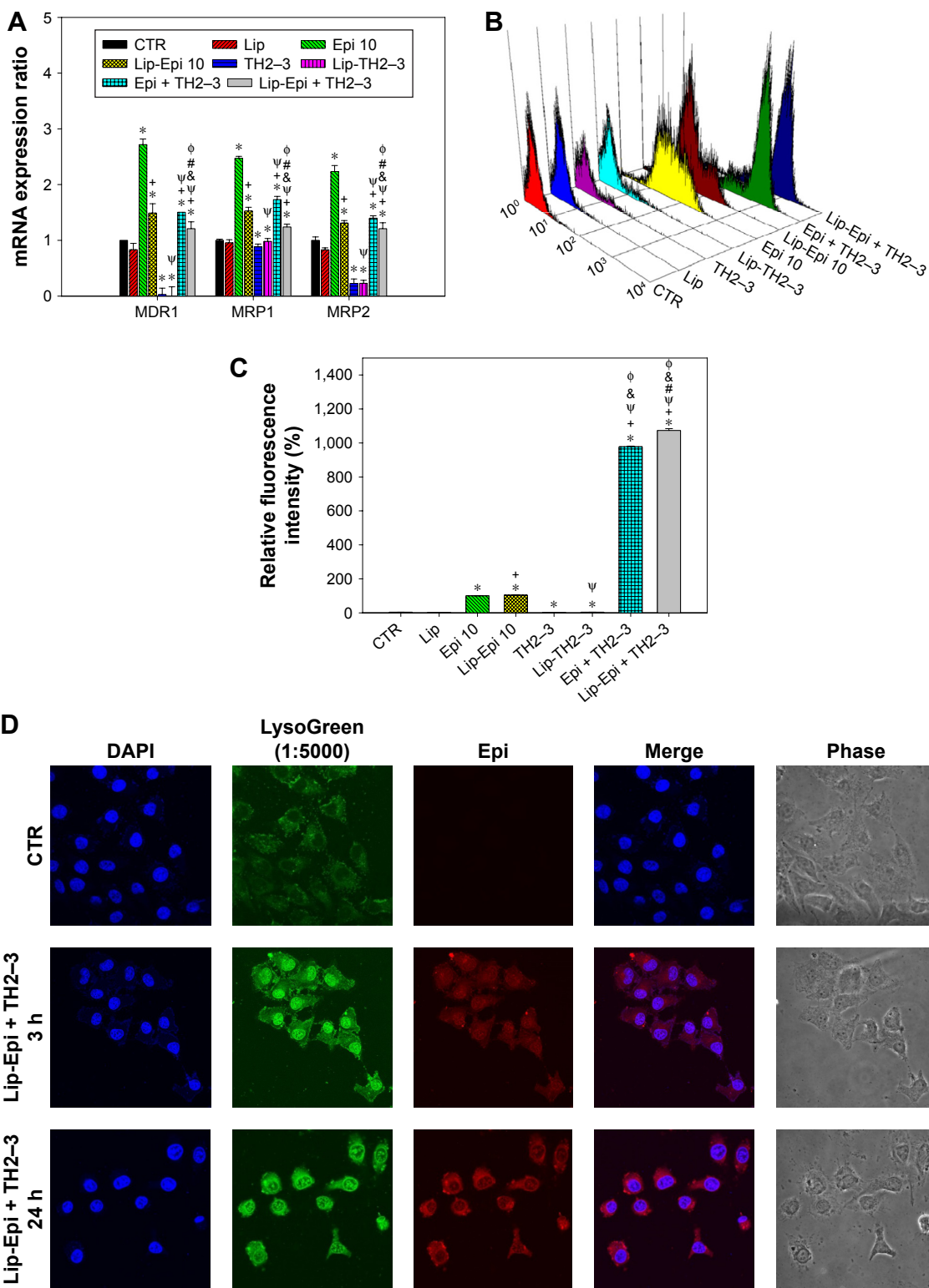
Figure 4 Effect of different treatments on the mRNA expressions and function of MDR transporters in HeLa cells.
