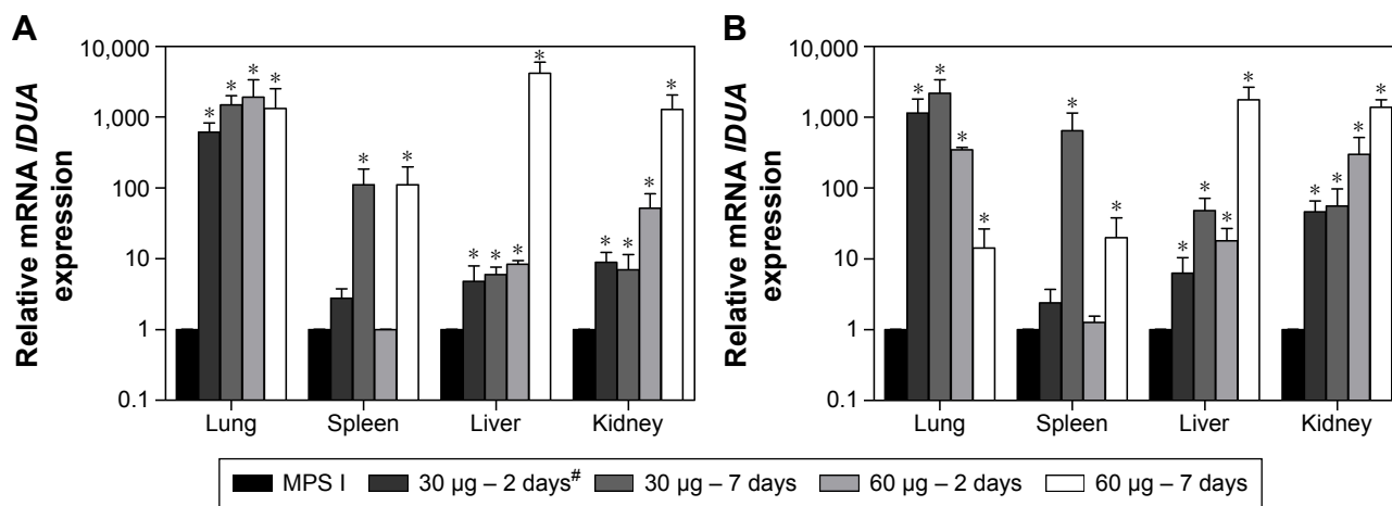
Figure 1 Relative expression of IDUA by real-time RT-qPCR in different organs of MPS I mice treated with NEP/pIDUA A (A) and NEP/pIDUA E (B). Notes: Mice were treated with 30 µg of pIDUA (dark gray bars) or 60 µg of pIDUA (light gray bars) and euthanized 2 days after intravenous injection or 30 µg of pIDUA (medium gray bars) or 60 µg of pIDUA (white bars) and euthanized 7 days after intravenous injection. Nontreated MPS I mice were used as control (black bars). Expression ratios are relative to GAPDH endogenous control. Values represent the mean ± standard error of the mean and are presented in log scale. *Difference between treated and nontreated MPS I mice (Student's t -test, P <0.05). #Data from Fraga et al. 7 Abbreviations: MPS I, mucopolysaccharidosis type I; RT-qPCR, quantitative real-time polymerase chain reaction.
