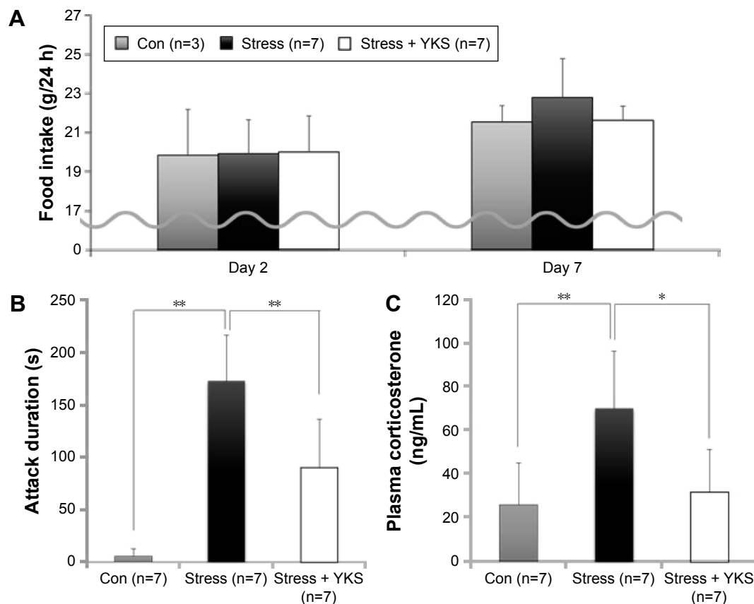
Figure 3 Effects of YKS on social isolation stress.
