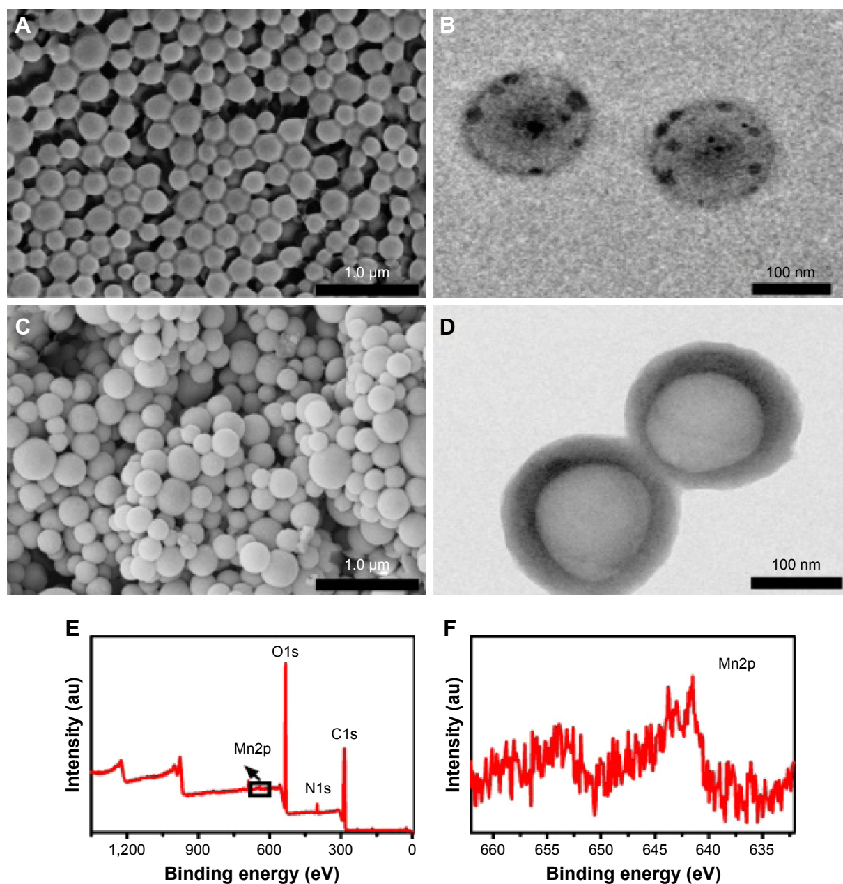
Figure 1 (A, C) SEM and (B, D) TEM images of (A, B) PLGA nanoparticles and (C, D) PDA@PLGA nanoparticles. XPS patterns of (E) Mn 2+ -PDA@PLGA and (F) corresponding deconvoluted Mn2p spectrum of Mn 2+ -PDA@PLGA; (F) is the enlarged view of black box in (E).
