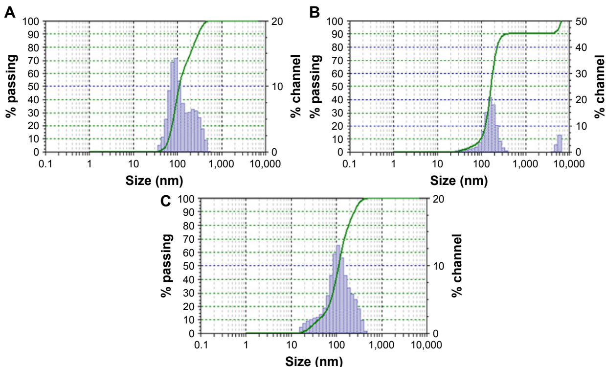
Figure 3 Distribution of particle size of AgNPs 1:100 (A), 1:50 (B), and 1:25 (C). Abbreviation: AgNPs, silver nanoparticles.
