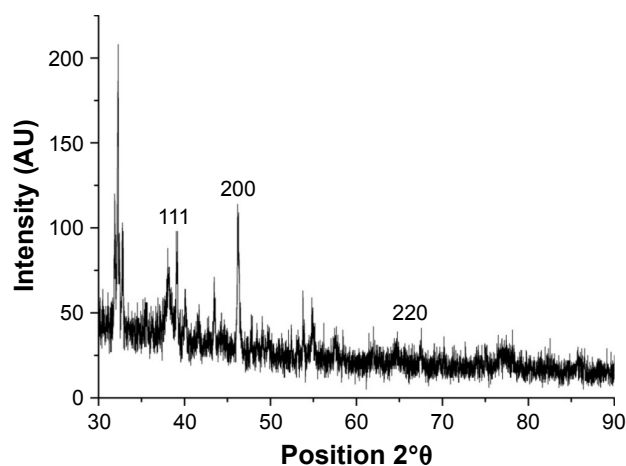
Figure 4 XRD spectra of biosynthesized AgNPs.
