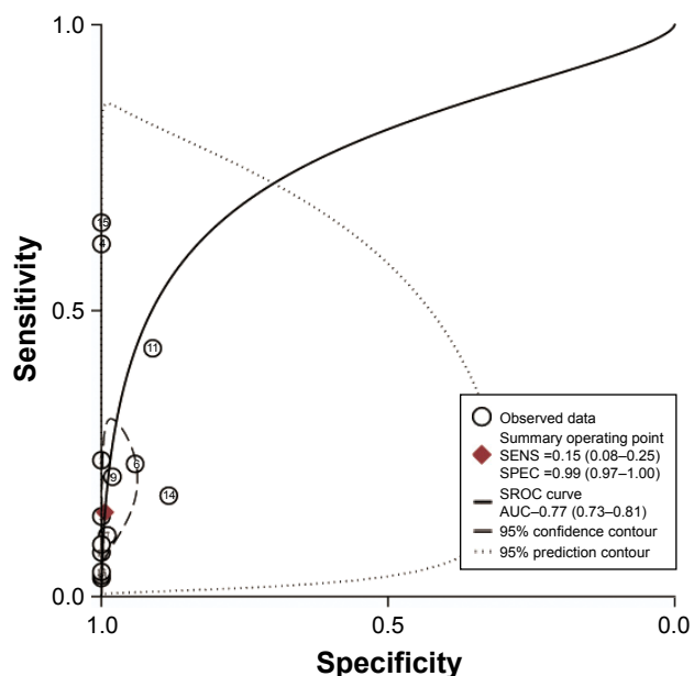
Figure 6 SROC plots of methylated MLHI for the diagnosis of esophageal cancer.
