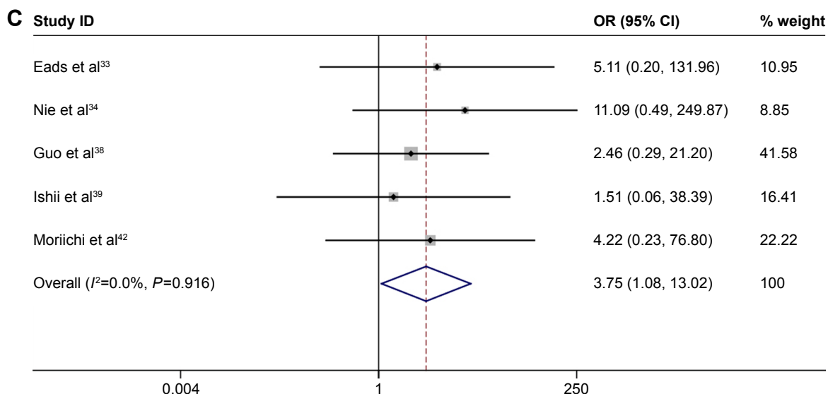
Figure 2 Pooled forest plot of MLHI methylation frequency during the carcinogenesis of esophageal cancer. Notes: (A) Carcinoma versus healthy controls: OR=8.40, 95% CI =5.75–12.28. (B) Carcinoma versus precancerous lesions: OR=3.08; 95% CI =1.64–5.92. (C) Precancerous lesions versus healthy controls: OR=3.75; 95% CI =1.08–13.02. Abbreviations: MLHI , mutL homolog-1; OR, odds ratio.
