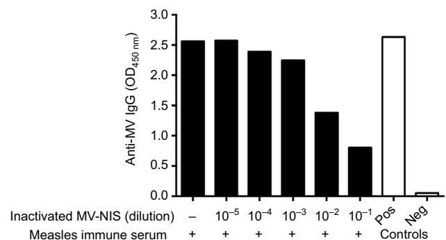
Figure 2 UV-inactivated MV-NIS remains antigenic.
