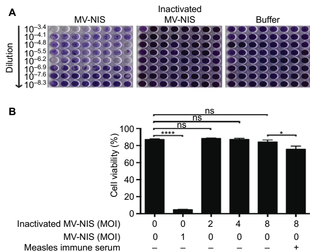
Figure 1 UV-inactivation abrogates replication of MV-NIS. MV-NIS was inactivated by 0.5 Joule/cm 2 UV-C light for 0.5 h.
