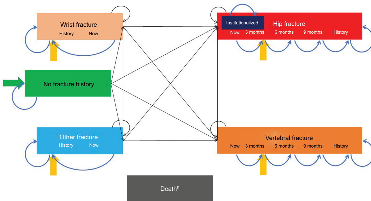
Figure 2 Markov model.
