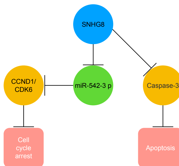
Figure 7 Schematic representation of the circuitry linking SNHG8, miR-542-3p, CCND1/CDK6, and cell cycle arrest or cell apoptosis.
