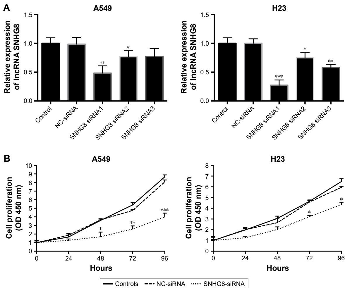
Figure 2 SNHG8 promotes NSCLC cells proliferation.
