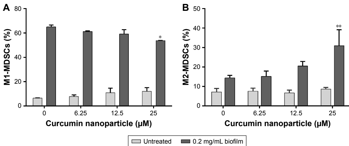
Figure 2 CURN induced expansion of MDSCs to M1- (A) and M2-phenotypic (B) MDSCs upon exposure to S. aureus biofilm via its anti-inflammatory activity. Notes: Data are expressed as the mean ± SD. * P < 0.05 and ** P < 0.01 compared to the biofilm-induced but no CURN treated group. Abbreviations: CURN, curcumin nanoparticles; MDSCs, myeloid-derived suppressor cells; S. aureus , Staphylococcus aureus .
