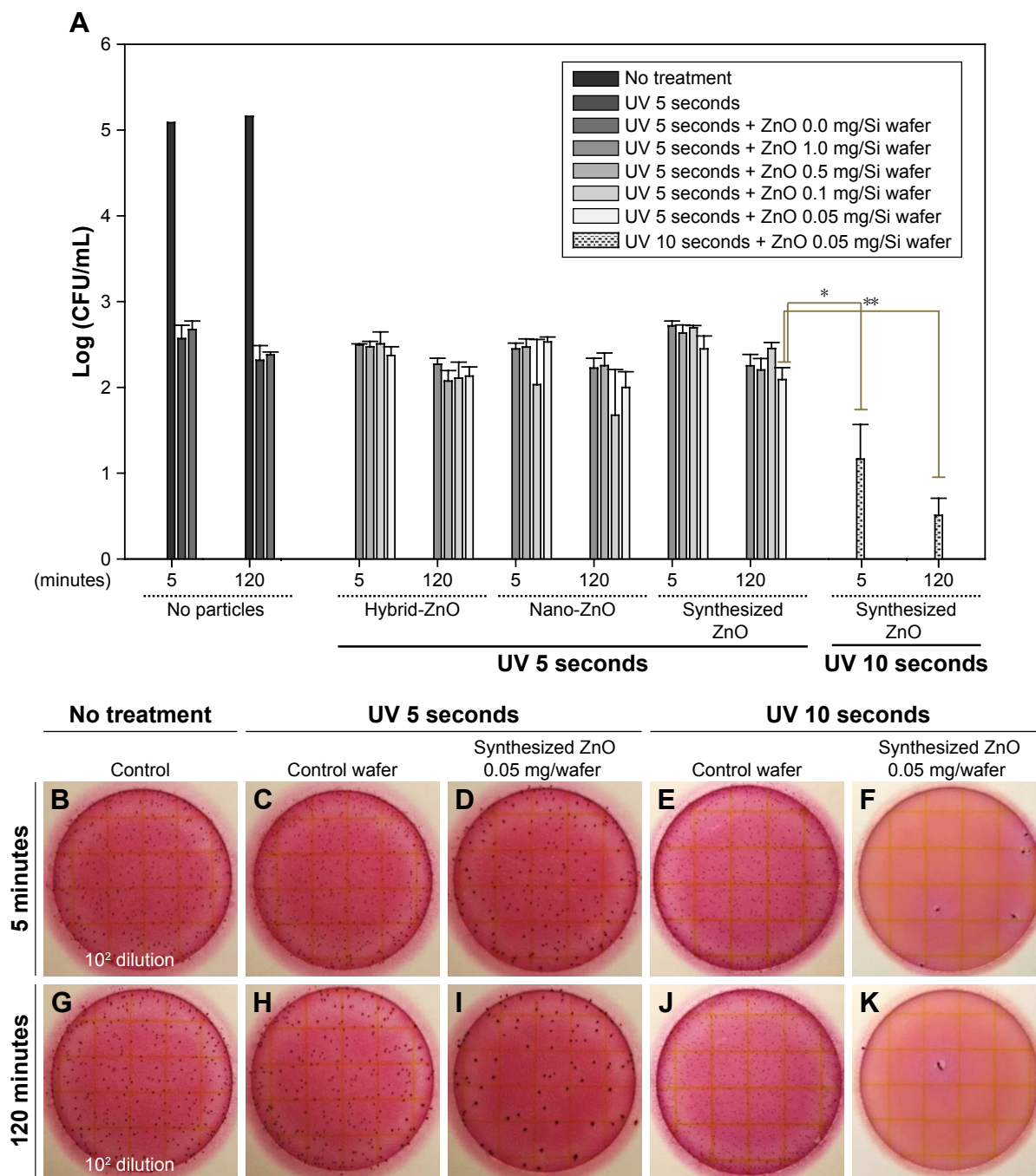
Figure 6 Antibacterial activity of the dual UV-irradiated ZnO nanoparticle network on Si wafer against Escherichia coli . Notes: (A) Plots of immobilized ZnO particle concentration vs log(CFU/mL). Representative plate images of (B and G) E. coli colonies ( 10^2 dilution) with no treatment, and E. coli colonies after dual UV irradiation for (C and H) 5 seconds and (E and J) 10 seconds and after dual UV-irradiated ZnO nanoparticle network (0.05 mg) treatment – UV irradiation for (D and I) 5 seconds and (F and K) 10 seconds; incubation for (B–F) 5 minutes and (G–K) 120 minutes. * P < 0.05 and ** P < 0.01 . Abbreviations: Si, silicon; UV, ultraviolet; ZnO, zinc oxide.
