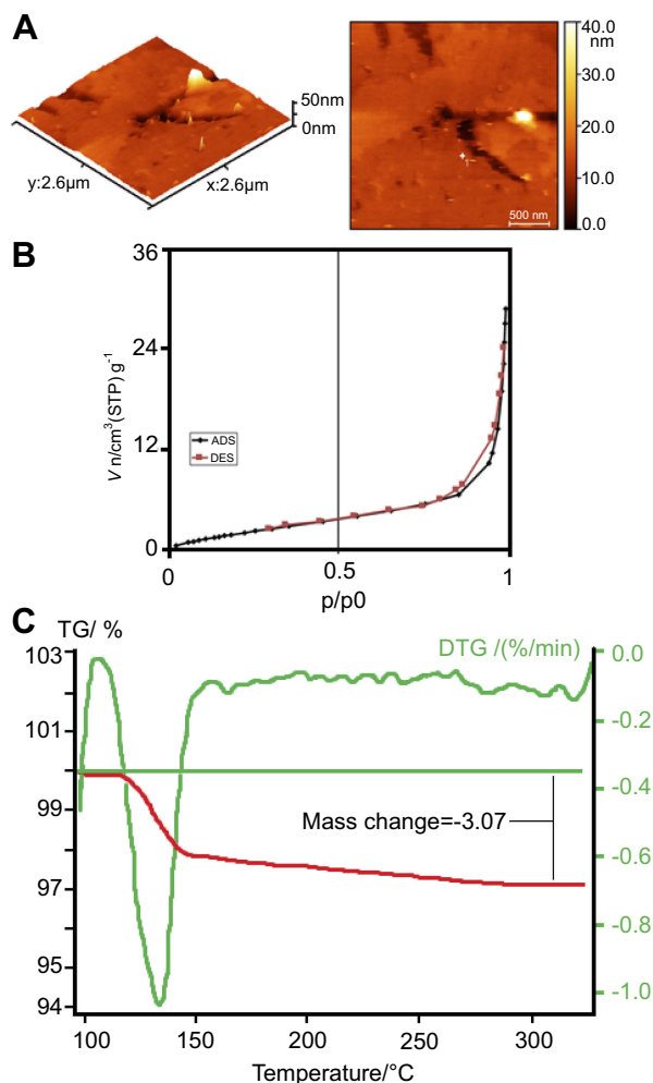
Figure 3 AFM images of the synthesized iron oxide quantum dots (A), the \text{N}_2 adsorption/desorption (ADS/DES) isotherm at room temperature (B), and TGA profile obtained for iron oxide quantum dots (C).
