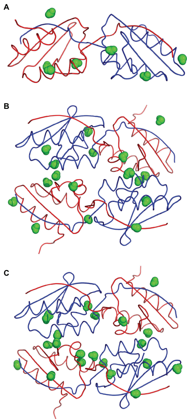
Figure 7 Water bridges observed in the MD simulations: A) sol_dimer , B) sol_tetra , C) cryst_tetra . The cuto3 distance for the detection of hydrogen bonds between water atoms and acceptor/donor groups was 2.5 Å. The Crh chains are colored in blue and red, and the water molecules are drawn in green CPK. This figure was realized with pymol 0.98. 51
