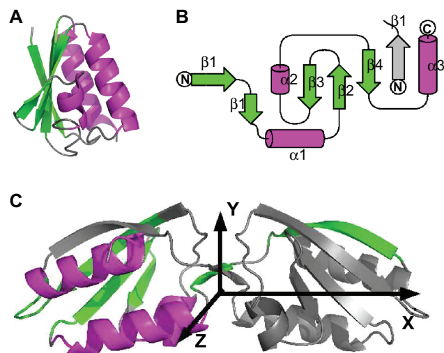
Figure 1 Structures of the Crh protein. A) The monomer structure determined by solution NMR (PDB entry: 1k1c) contains three \alpha helices ( \alpha 1 : residues 17–28, \alpha 2 : residues 47–50 and \alpha 3 : residues 70–83) as well as a \beta sheet formed from four \beta strands ( \beta 1 : residues 3–9, \beta 2 : residues 31–37, \beta 3 : residues 40–42 and \beta 4 : residues 60–67). B) Topology of a Crh monomer, inside the dimer, C) Dimer structure determined by X-ray crystallography (PDB entry: 1mo1). The \beta strands are in green and the \alpha helices in magenta. In the dimer (b,c), one monomer is colored and the other one displayed in gray. In c, the axes X, Y, Z allowing to define the angles \Psi , \Theta and \Phi are drawn. This figure was realized with pymol 0.98 51 and TopDraw. 52
