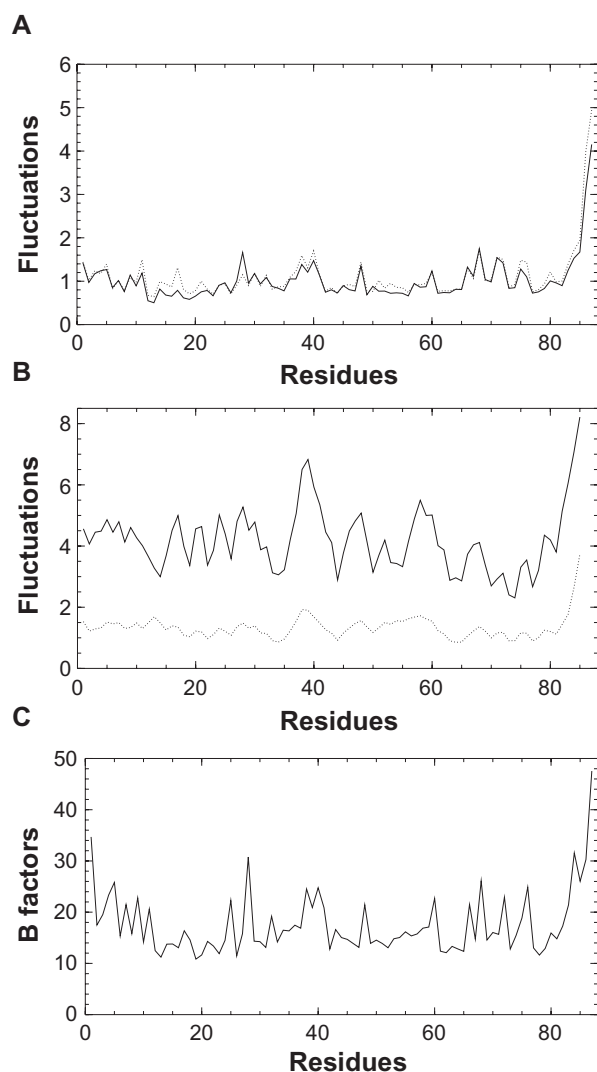
Figure 4 Comparison of the A ) fluctuations by residues in MD simulations ( cryst_tetra : solid, sol_tetra : dotted), of B ) the mean local RMSD among ARIA conformers (geometric force field: solid, water and NCS refinements: dotted) plotted along the sequence, and of C ) the mean B factors in the four chains of 1mo1.
