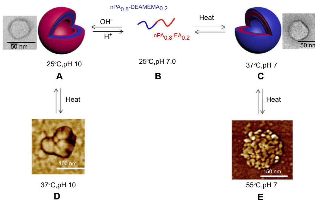
Figure 10 Self-assembling process of poly( nPA_{0.8} -co-DEAEMA _{0.2} )-block-poly( nPA_{0.8} -co-EA _{0.2} ) into vesicles, and then aggregates upon heating. Reprinted with permission from Savoji MT, Strandman S, Zhu XX. Switchable vesicles formed by diblock random copolymers with tunable pH- and thermo-responsiveness. Langmuir . 2013;29(23):6823–6832. Copyright 2013, American Chemical Society. 84
