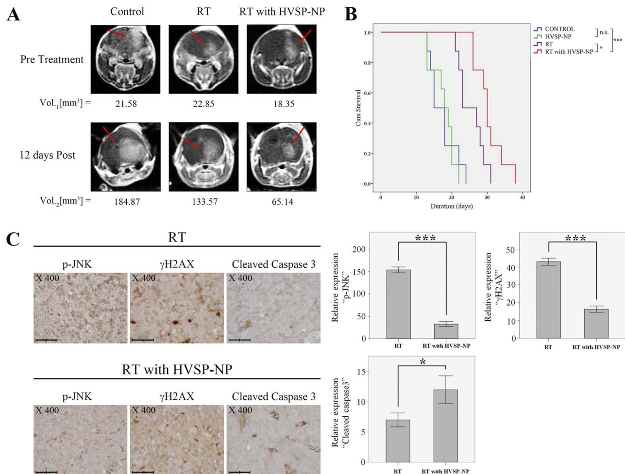
Figure 4 Survival studies for mice receiving various treatments. (A) MRI follow-up images. Tumor volume was measured using Leksell GammaPlan® (LGP, Dedicated treatment planning tool specifically designed for stereotactic radiosurgery). Red arrows indicate the presence of tumors. (B) Kaplan-Meier survival curves. (C) Immunohistochemistry staining results for p-JNK, \gamma H2AX, and Cleaved Caspase-3 in extracted mouse brain tumors. Each immunoreactivity pattern was confirmed by quadruplicate specimens from the same mouse. Scale bar, 10 \mu m. Histograms showing the quantitative analysis of p-JNK, \gamma H2AX and Cleaved Caspase3 expression levels for RT \pm HVSP-NP. Error bars indicate \pm SD; columns, mean.
