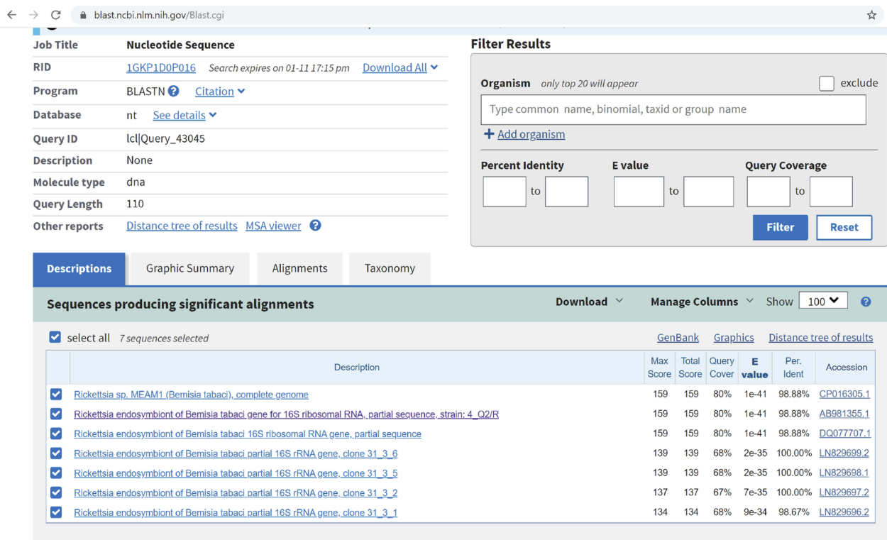
Figure 4 Alignment of the PCR product sequence of 16srRNA of Rickettsia Endosymbiont Besimisia Tabaci with submitted sequences for the same pathogen in NCBI.
