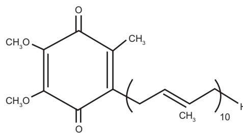
Ubiquinone (2,3-Dimethoxy-5-methyl-6-decaprenyl-1,4-benzoquinone)
