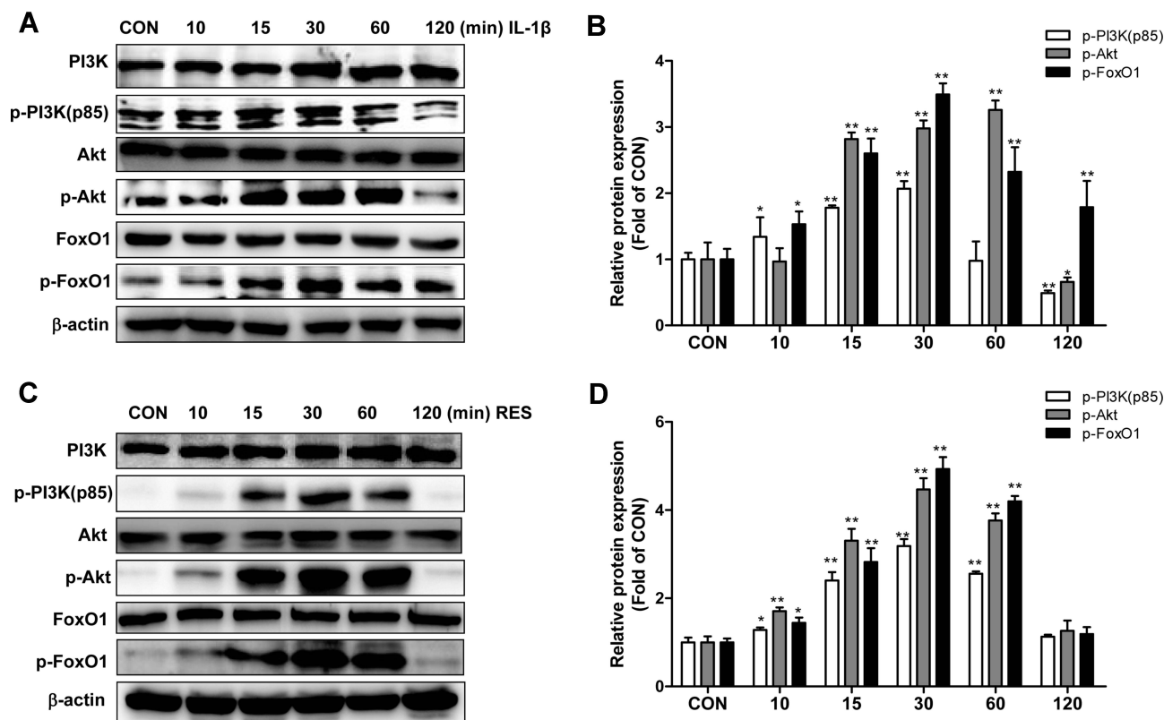
Figure 2 IL-1β or resveratrol treatment promoted activation of the PI3K/Akt signaling but led to inactivation of FoxO1 in SW1353 cells. (A), (C) Serum-starved (0.5% FBS) SW1353 cells were treated with 10 ng/mL IL-1β or resveratrol (50 μM) for 10, 15, 30, 60 and 120 min. p-PI3K, p-Akt, and p-FoxO1 expression were determined by Western blot analysis. (B), (D) The levels of p-PI3K, p-Akt, p-FoxO1 were normalized with their respective total PI3K, Akt, FoxO1 levels. The results for Western blot were expressed as folds of CON. Data were expressed as the mean ± SD of three independent experiments. *P <0.05, **P <0.01 versus the CON group.
