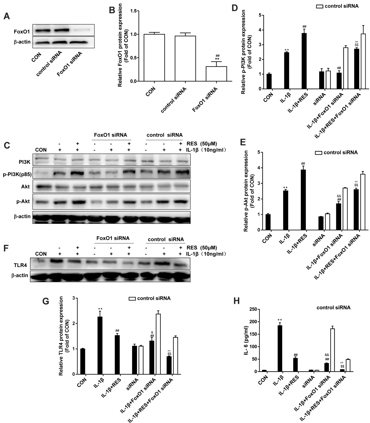
Figure 5 FoxO1-knockdown decreased p-PI3K, p-Akt and TLR4 protein expression in IL-1β-treated SW1353 cell. (A) SW1353 cells were transfected with FoxO1 siRNA (50 nM) or control siRNA for 48 h, FoxO1 expression was analyzed by Western blot. (B) The levels of FoxO1 were normalized with β-actin. The results for Western blot were expressed as folds of CON. ** P < 0.01, versus the CON, ### P < 0.01 versus control siRNA. (C), (F) After SW1353 cells were transfected with FoxO1 siRNA for 48 h as described above, cells were exposed to 10 ng/mL IL-1β with or without 50 μM RES for 30 min or 24 h, p-PI3K, p-Akt, and TLR4 expression was analyzed by Western blot. (D–E), (G) The levels of p-PI3K, p-Akt, and TLR4 were normalized with their respective total PI3K, Akt or β-actin levels. The results for Western blot were expressed as folds of CON. (H) IL-6 concentrations in the culture supernatants were assessed by ELISA. All data above were expressed as the mean ± SD of three independent experiments. ** P < 0.01 versus the CON, ### P < 0.01 versus the IL-1β, $$$ P < 0.01 versus IL-1β + RES, &# P < 0.05, && P < 0.01 versus siRNA, ^^ P < 0.01 versus siRNA + IL-1β.
