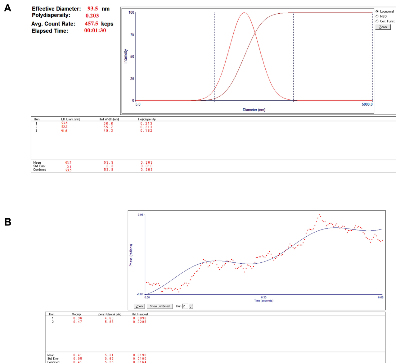
Figure 1 Physicochemical characteristics of formulation of Ginsenoside Rh2-loaded nanionosome with DOTAP. (A) The size distribution and PDI formulation of Ginsenoside Rh2-loaded nanionosome with DOTAP. (B) The zeta potential formulation of Ginsenoside Rh2-loaded nanionosome with DOTAP.
