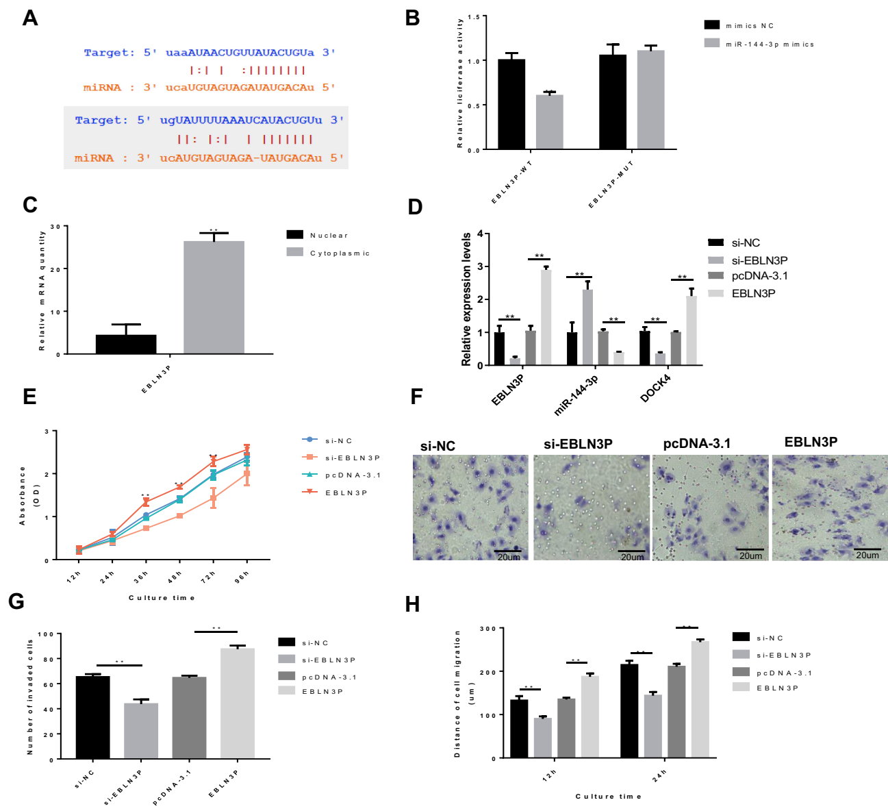
Figure 1 EBLN3P knockdown inhibits the proliferation, migration and invasion of liver cancer cells in vitro. HepG2 cells were transfected with EBLN3P -targeted siRNA (si- EBLN3P ), negative control siRNA (si-NC), pcDNA3.1- EBLN3P overexpression vector (pcDNA- EBLN3P ) or blank vector plasmid (pcDNA-3.1). (A) Bioinformatics analysis demonstrated that EBLN3P can directly interact with miR-144-3p (up) and that miR-144-3p can directly bind to the 3'-UTR regions of DOCK4 (down). (B) Dual-luciferase reporter assays were performed to verify the impact of miR-144-3p on the luciferase signal of reporter plasmids containing EBLN3P . (C) The nuclear and cytoplasmic expression levels of EBLN3P in HepG2 cells. (D) The expression levels of EBLN3P and miR-144-3p were explored via reverse transcription-quantitative PCR. (E) Cell proliferation was tested by the Cell Counting Kit-8 assay. (F) The number of invaded cells. (G) Cell invasion was detected by the Transwell assay. (H) Cell migration was detected by the wound healing assay. That data is shown as the mean \pm SD. ** P < 0.01 .
