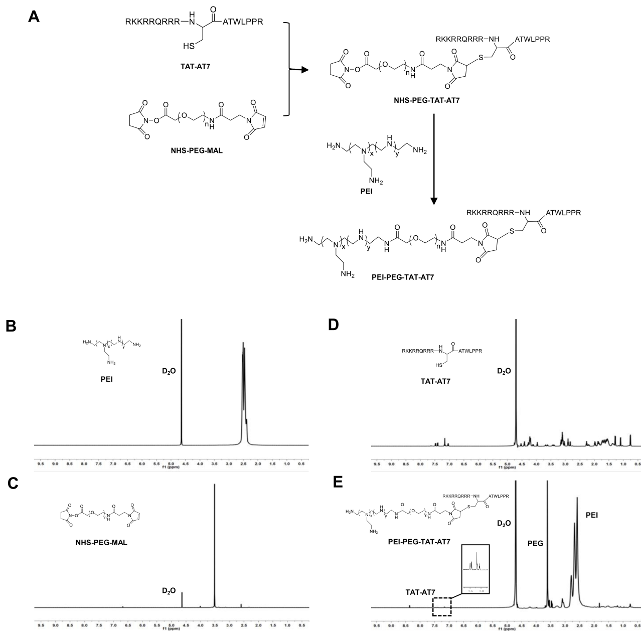
Figure 4 The synthetic mechanism and 1 H-NMR spectrum of PEI-PEG-TAT-AT7 (PPTA). (A) The whole process of PPTA synthesis was divided into two steps as presented. (B–E) 1 H NMR spectra of PEI, TAT-AT7, NHS-PEG-MAL, and PPTA.
