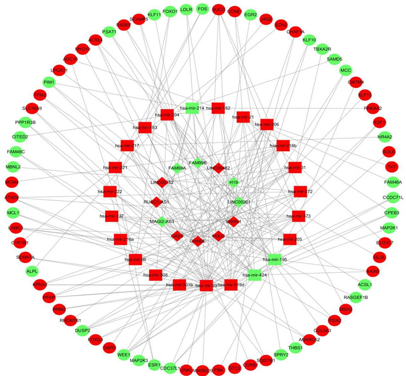
Figure 3 The lncRNA-miRNA-mRNA ceRNA network in AFP-negative HCC. The diamond represents lncRNA, the square represents miRNA and the circle denotes mRNA. The red nodes indicate upregulated RNAs and the green nodes indicate downregulated RNAs.
