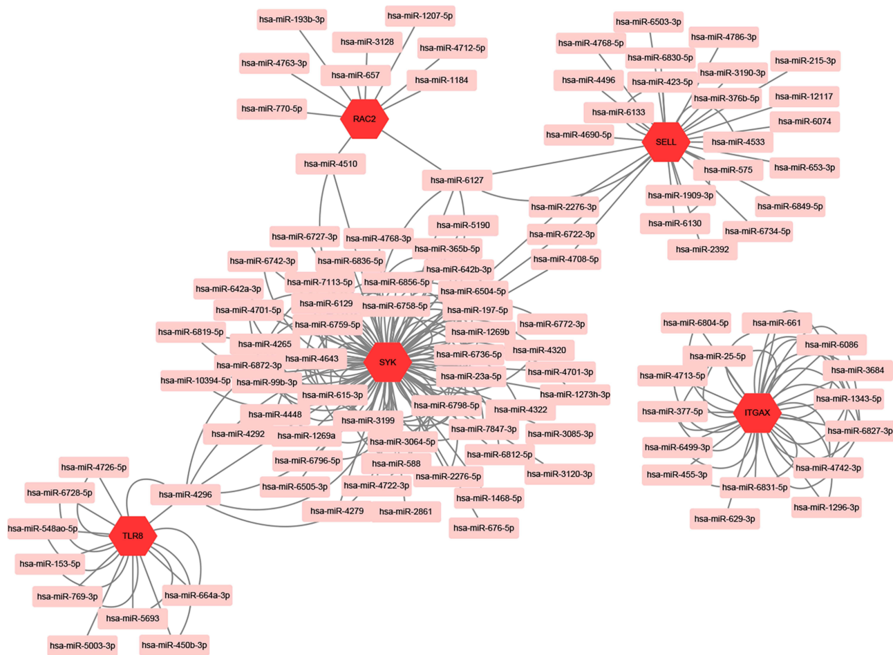
Figure 9 mRNA-miRNA regulation network of hub genes was constructed by MiRwalk.
