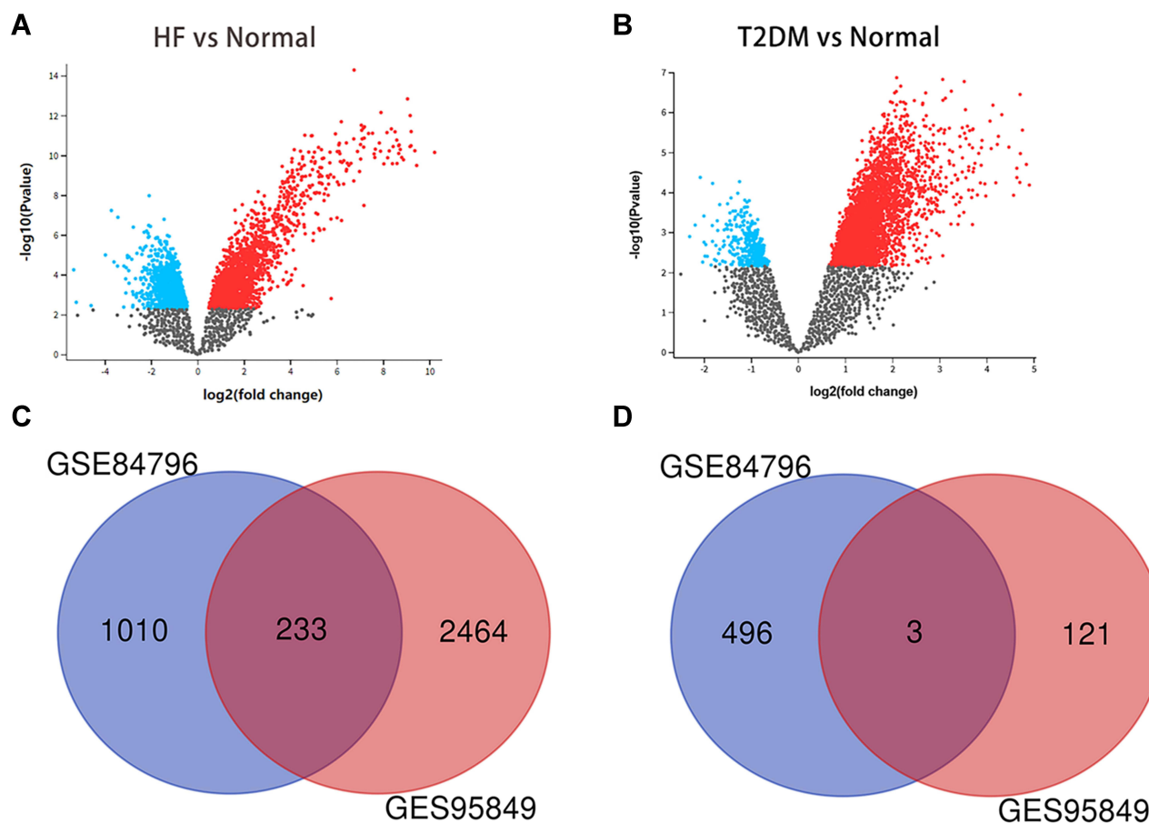
Figure 2 Identification of differentially expressed genes in the two datasets. (A) Volcano plot of HF microarray data. (B) Volcano plot of T2DM microarray data. (C) Venn diagram of the 233 communal upregulated DEGs in HF and T2DM. (D) Venn diagram of the 3 communal downregulated DEGs in HF and T2DM.
