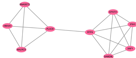
Figure 5 Top modules from the protein–protein interaction network. (A) Module A and the enriched pathways of module by KOBAS 3.0. (B) Module B and the enriched pathways of module by KOBAS 3.0. (C) Module C and the enriched pathways of module by KOBAS 3.0. (D) Module D and the enriched pathways of module by KOBAS 3.0.
