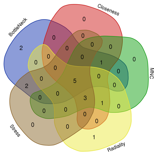
Figure 6 Five hub genes were identified by overlapping the first 10 genes in the five classification methods of cytoHubba.
