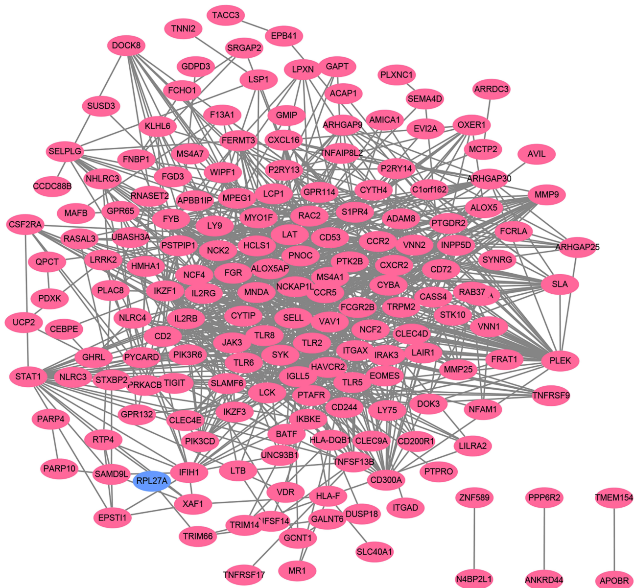
Figure 4 Based on database STRING and Cytoscape software, PPI networks of the DEGs were constructed. The red point represents upregulated genes, and blue point represents downregulated genes.
