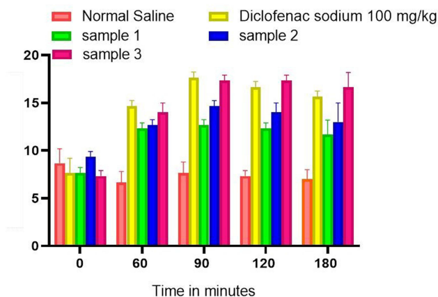
Figure 2 Analgesic activity of polyherbal extracts (GCTC) by tail flick method.
