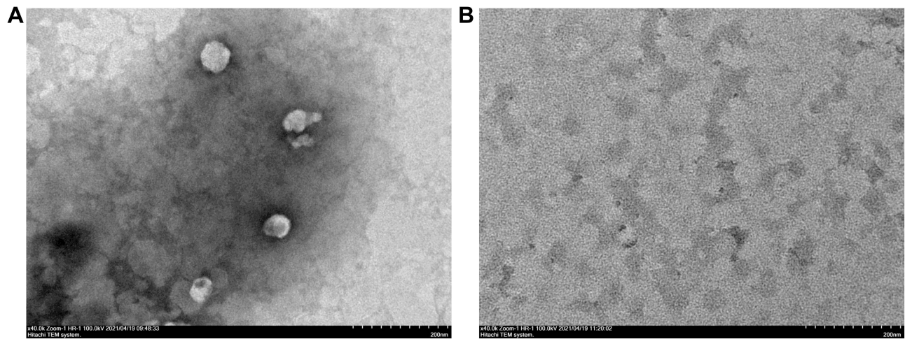
Figure 2 TEM images of M/LST without (A) and with (B) H_2O_2 .
