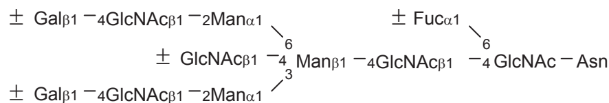
Figure 2 Fc-Linked oligosaccharides of antibodies. A conserved oligosaccharide core, linked to the Asn-297, is composed of a mannosyl-chitobiose core structure in the presence or absence of a core fucose (Fuc), a bisecting N-acetylglucosamine (GlcNAc) and terminal galactose (Gal) and sialic acid; this structure gives rise to heterogeneity with a mixture of 30 or more glycoforms.
