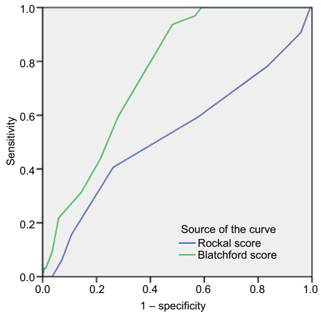
Figure 5 The area under the ROC curve to determine the value of GBS (0.757, cutoff =6.5, sensitivity: 93.8%, specificity: 51.8%) and full RS (0.528, cutoff =2.5, sensitivity: 71.8%, specificity: 51.8%) for predicting need for transfusion.
