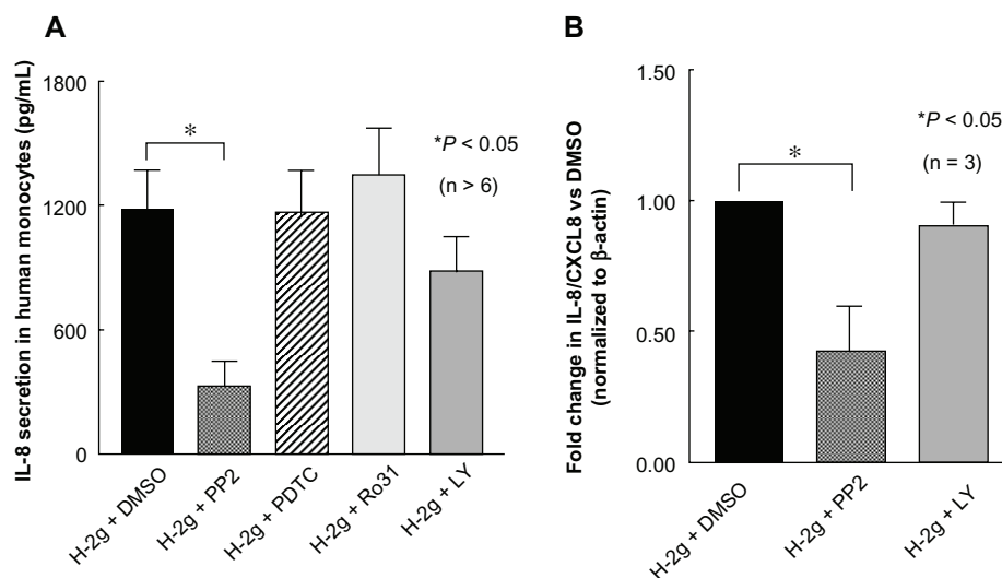
Figure 2 Src is required for H-2g induced MN production of IL-8/CXCL8. (A) Isolated MNs were cultured in the presence of H-2g with DMSO (vehicle control), PP2 529573 (Src inhibitor), PDTIC (NF- \kappa B inhibitor), Ro31 (PKC inhibitor), or LY294002 (PI3K inhibitor). Cell culture supernatants were collected and subject to an ELISA to determine the amount of IL-8/CXCL8. (B) Isolated MNs were cultured in the presence of H-2g with DMSO (vehicle control), PP2 529573 (Src inhibitor), or LY294002 (PI3K inhibitor).
