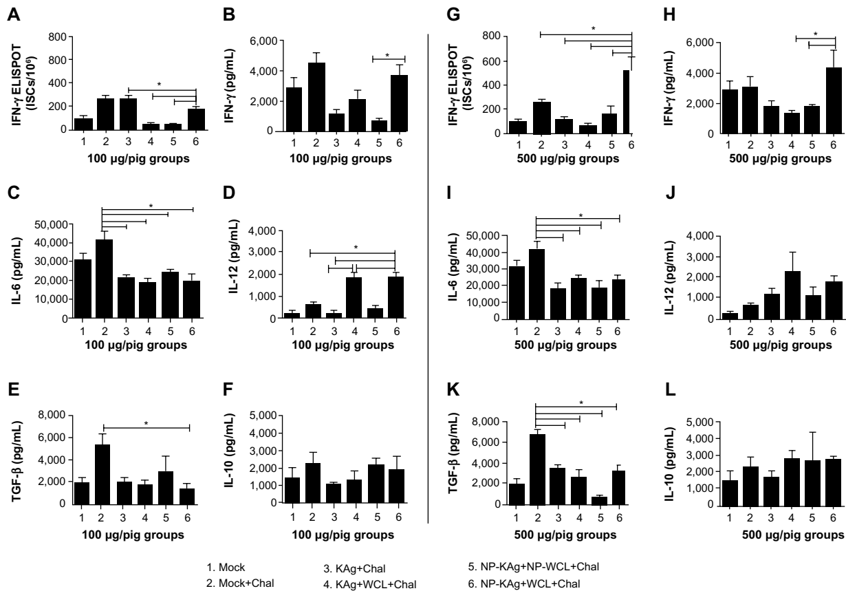
Figure 4 Enhanced frequency of IFN- \gamma secreting cells (A and G) and upregulated production of Th1 (IFN- \gamma and IL-12) and reduced immunosuppressive cytokines (TGF- \beta and IL-10) in pigs vaccinated with adjuvanted NP-KAg vaccine (B-F and H-L).
