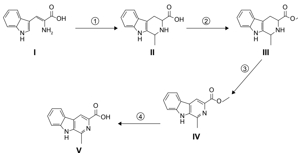
Scheme 1 Synthesis of 1-methyl- \beta -caboline-3-carboxylic acid.
