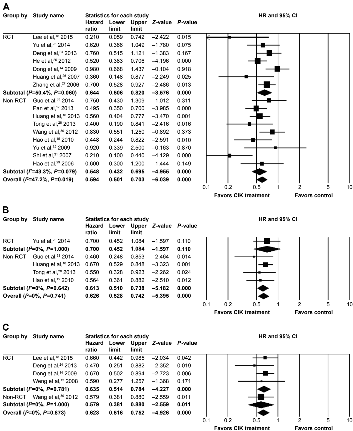
Figure 3 Meta-analysis for treatment effect on (A) OS, (B) PFS, and (C) DFS/RFS. Abbreviations: CI, confidence interval; CIK, cytokine-induced killer; DFS, disease-free survival; HR, hazard ratio; OS, overall survival; RFS, recurrence-free survival; RCT, randomized controlled trial.
