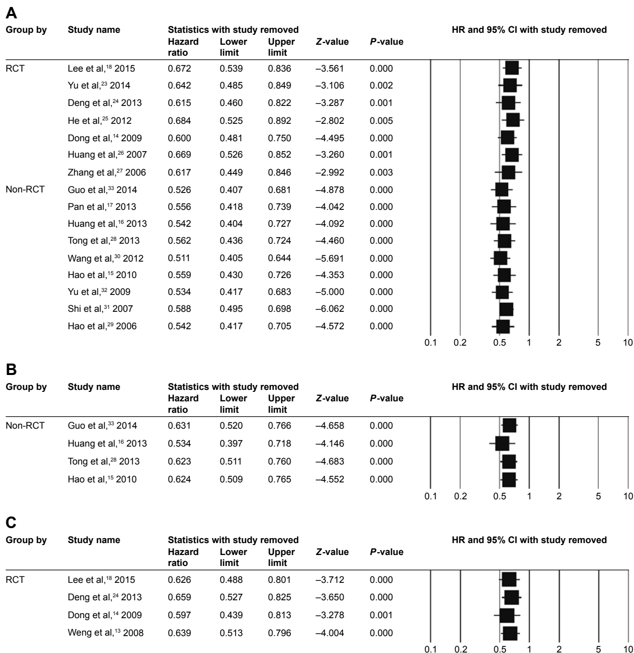
Figure 4 Sensitivity-analysis for treatment effect on (A) OS, (B) PFS, and (C) DFS/RFS.
