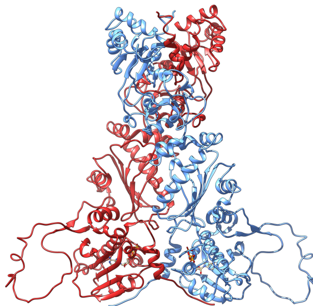
Figure 1 Structural model of T. rubrum Hsp90 dimeric structure generated using as a template the crystal structure of Hsp90 from Saccharomyces cerevisiae (PDB ID: 2CG9). Notes: Blue and red colors indicate the 2 monomers. This image has been generated using the Chimera program. 42 Abbreviation: PDB, Protein Data Bank.
