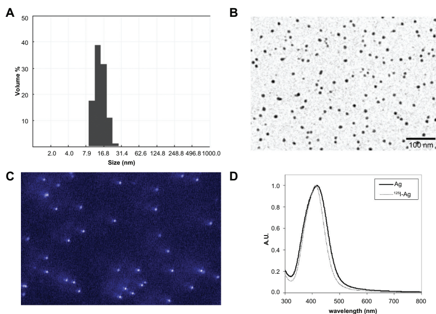
Figure 1 Characterization of synthesized silver nanoparticles (Ag NPs). A ) Size distribution profile of ^{125}\text{I} -Ag NPs as analyzed by photon correlation spectroscopy. B ) Transmission electron microscopy (TEM) of ^{125}\text{I} -Ag NPs. C ) Light scattering as observed under a dark field real-time microscope (RTM). D ) Absorption spectroscopy comparing Ag NPs and ^{125}\text{I} -Ag NPs showed that the characteristic plasmon band for Ag NPs was not significantly altered after radiolabeling.
