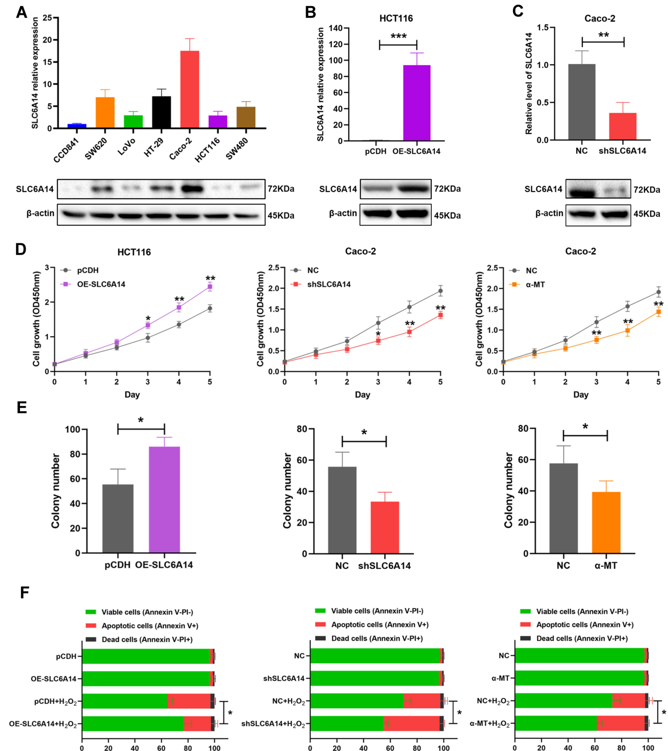
Figure 3 SLC6A14 facilitates cell proliferation and inhibits cell apoptosis in vitro. (A) SLC6A14 expression level was detected in a series of CRC cell lines and normal colonic epithelial cell line by qRT-PCR and immunoblot. (B, C) The overexpression and knockdown efficiency of SLC6A14 were examined by qRT-PCR and immunoblot. (D) CCK-8 assay was performed to access the effects of modulating SLC6A14 on cell proliferation of CRC cells. (E) Colony-forming assays in SLC6A14 overexpression and depletion CRC cells were conducted. (F) The percentage of cell apoptosis after regulating SLC6A14 expression was determined by flow cytometric analysis. *P < 0.05, **P < 0.01, and ***P < 0.001. Bars in all graphs represented mean ± S.D.
