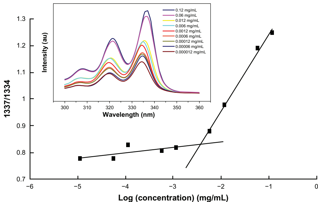
Figure 4 Plots of 1337/1334 versus log C of copolymer. Note: Inset: the excitation spectra of PEG-PRL solution with different concentrations in the presence of pyrene take PEG-PRL2 copolymer as representative. Abbreviations: PEG, poly(ethylene glycol); PRL, poly(racemic-leucine).
