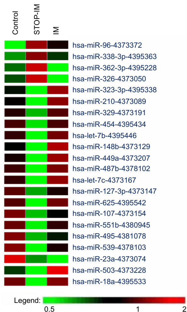
Figure 1 miRNA profiling by TaqMan (Thermo Fisher Scientific, Waltham, MA, USA) miRNA array.
