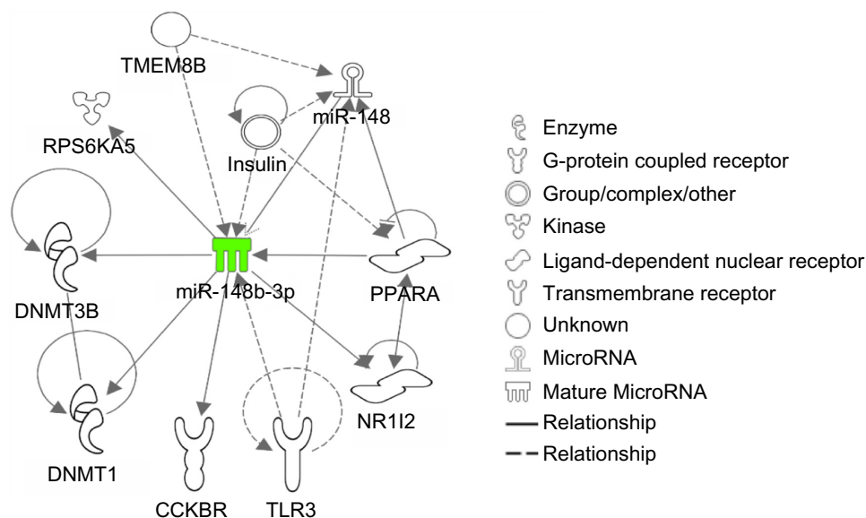
Figure 3 Network analysis of miR-148b by Ingenuity Pathways Analysis.
