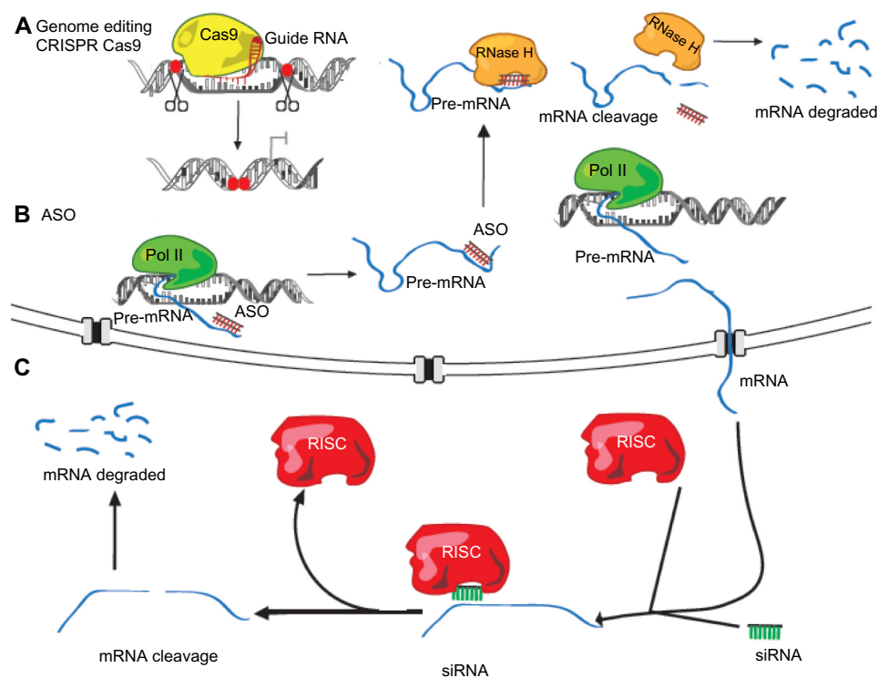
Figure 3 IncRNA loss-of-function strategies.
