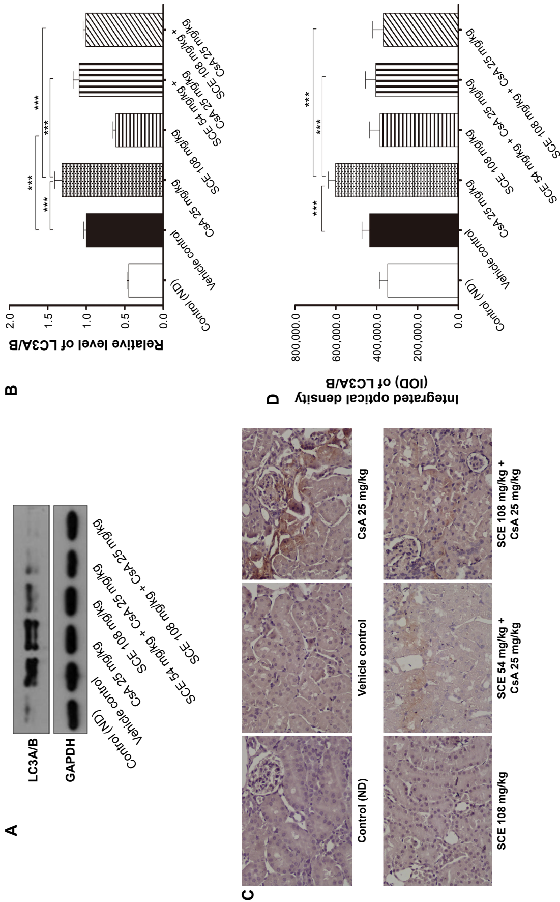
Figure 12 Effect of SCE on the expression of LC3A/B in CsA-induced nephrotoxicity.
