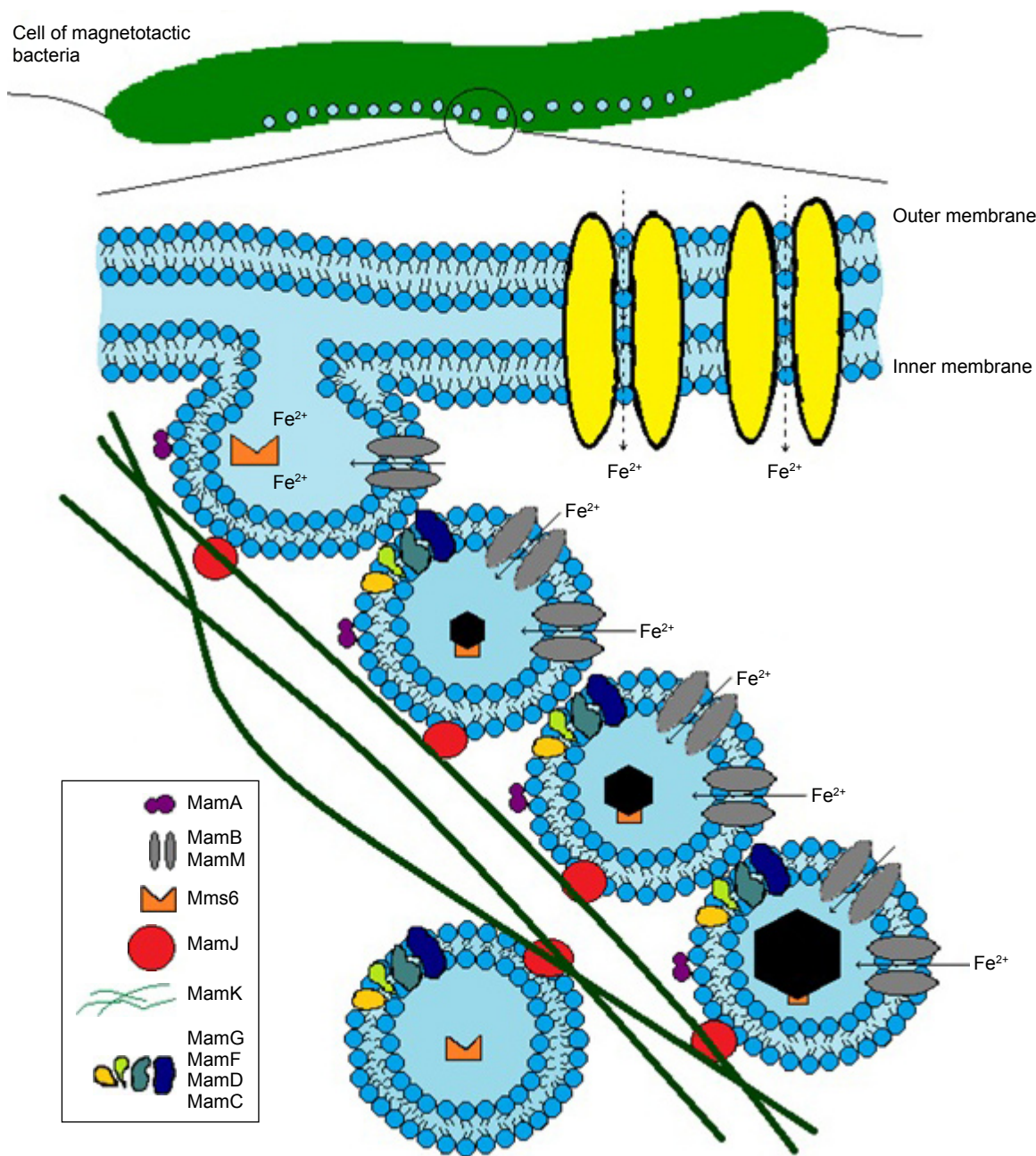
Figure 5 Schematic representation of BMNP biomineralization in magnetotactic bacteria. Note: Black hexagonal symbols represent magnetic crystal growth inside magnetosome vesicles. Abbreviation: BMNP, biogenic magnetic nanoparticle.
