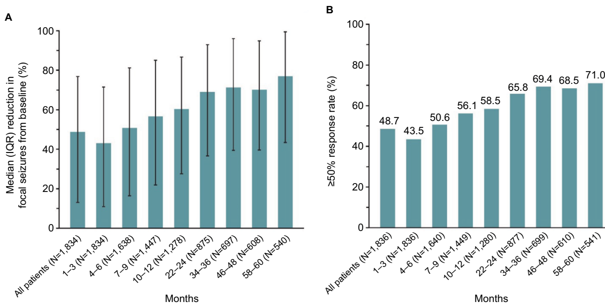
Figure 8 Seizure reduction and responder rates. (A) Median (IQR) percentage reduction in focal seizures from baseline; (B) \geq 50\% responder rates over time for BRV modal doses 50–200 mg/day in pooled long-term follow-up analysis.
