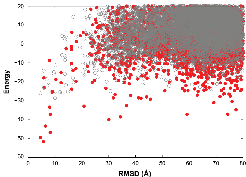
Figure 6 Energy landscape for the IB6C complex before (pyDock values in gray) after side chain minimization and global energy minimization (ie, including backbone and side-chains) with UNRES forcefield 07 \alpha\beta (in red).
