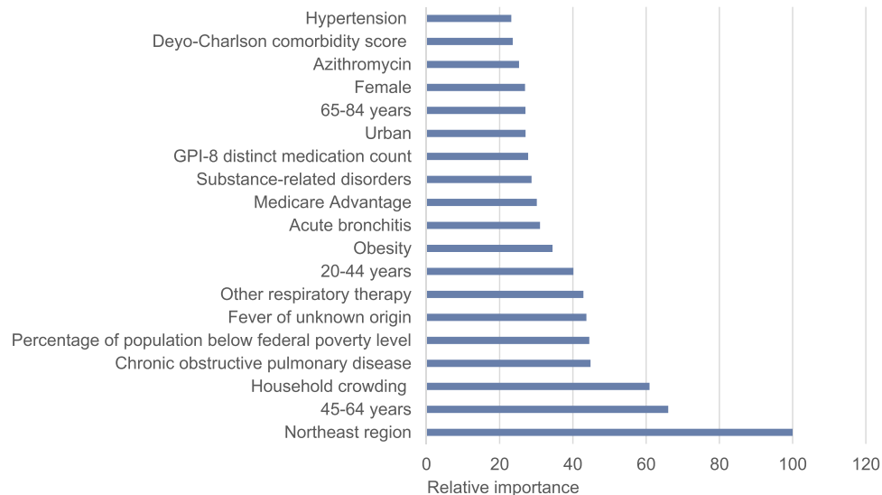
Figure 1 Importance ranking of the twenty most influential predictors from the gradient boosting model.
