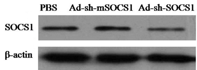
Figure 1 Western blot analysis of SOCS1 silencing. SOCS1 and \beta -actin proteins were identified using anti-SOCS1 polyclonal and anti- \beta -actin monoclonal antibodies (Santa Cruz Biotechnology, Santa Cruz, CA, USA), respectively.
