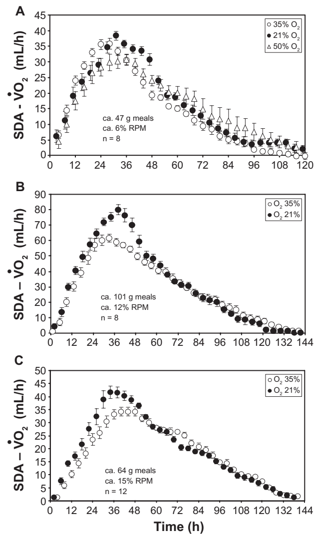
Figure 3 Specific dynamic action responses under normoxia and hyperoxia in pitvipers measured during the three experiments. A) Snakes (n = 8) ingesting approximately 47 g mouse meals subjected to three O 2 treatment levels. B) Snakes (n = 8) ingesting approximately 101 g mouse meals subjected to two O 2 treatment levels. C) Snakes (n = 12) ingesting approximately 64 g mouse meals subjected to two O 2 treatment levels. Error bars refer to ± one standard error of the mean. For clarity, data points are slightly offset along the x-axis.
