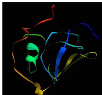
Figure 5 Homology based model of OMPs of E. tarda (DOZFR4).
