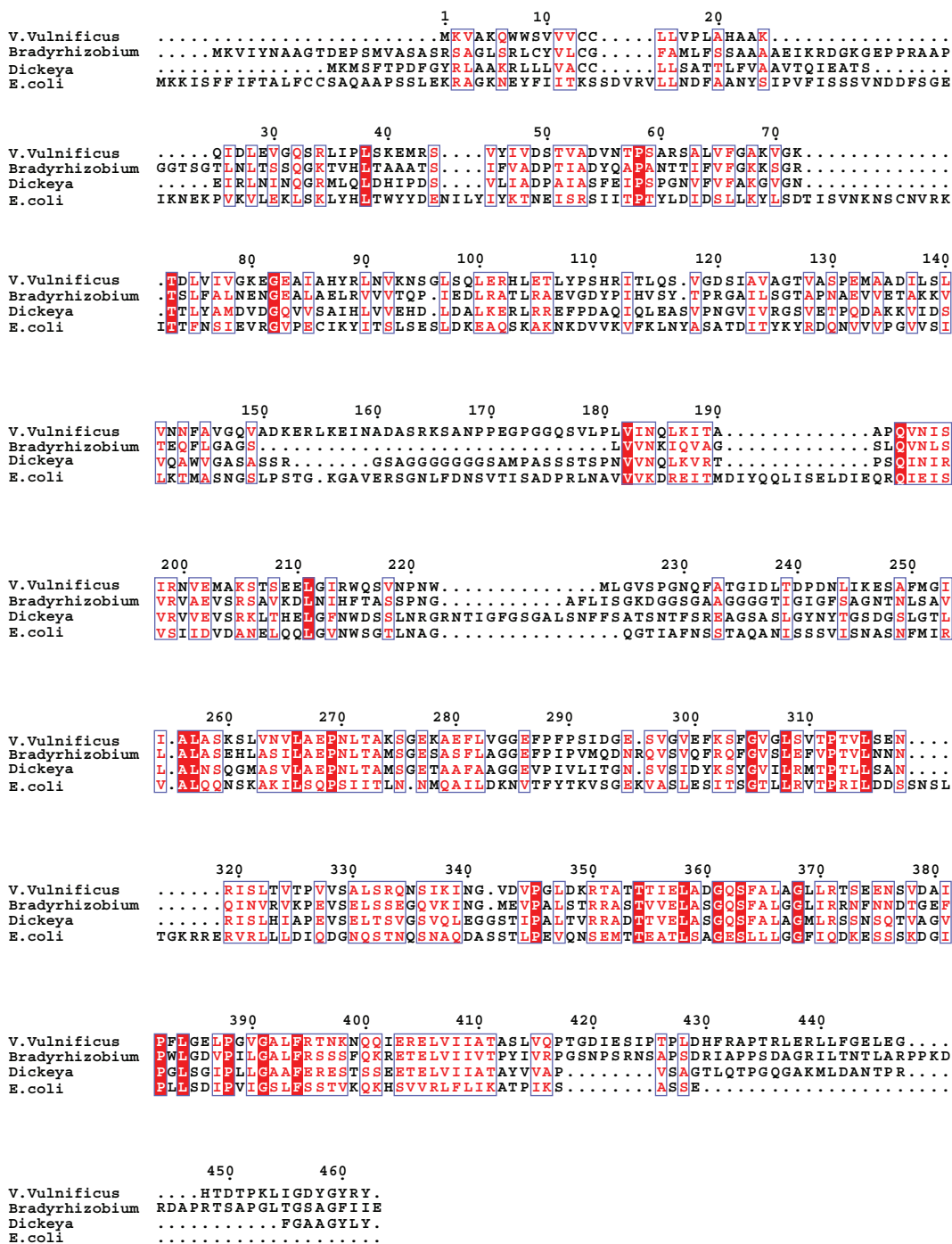
Figure 1 Multiple alignment of secretin of Vibrio vulnificus ( V. vulnificus ), Bradyrhizobium , E. coli and Dickeya zeae ( Erwinia chrysanthemi ). Identical residues colored white in red background and similar residues colored red.
