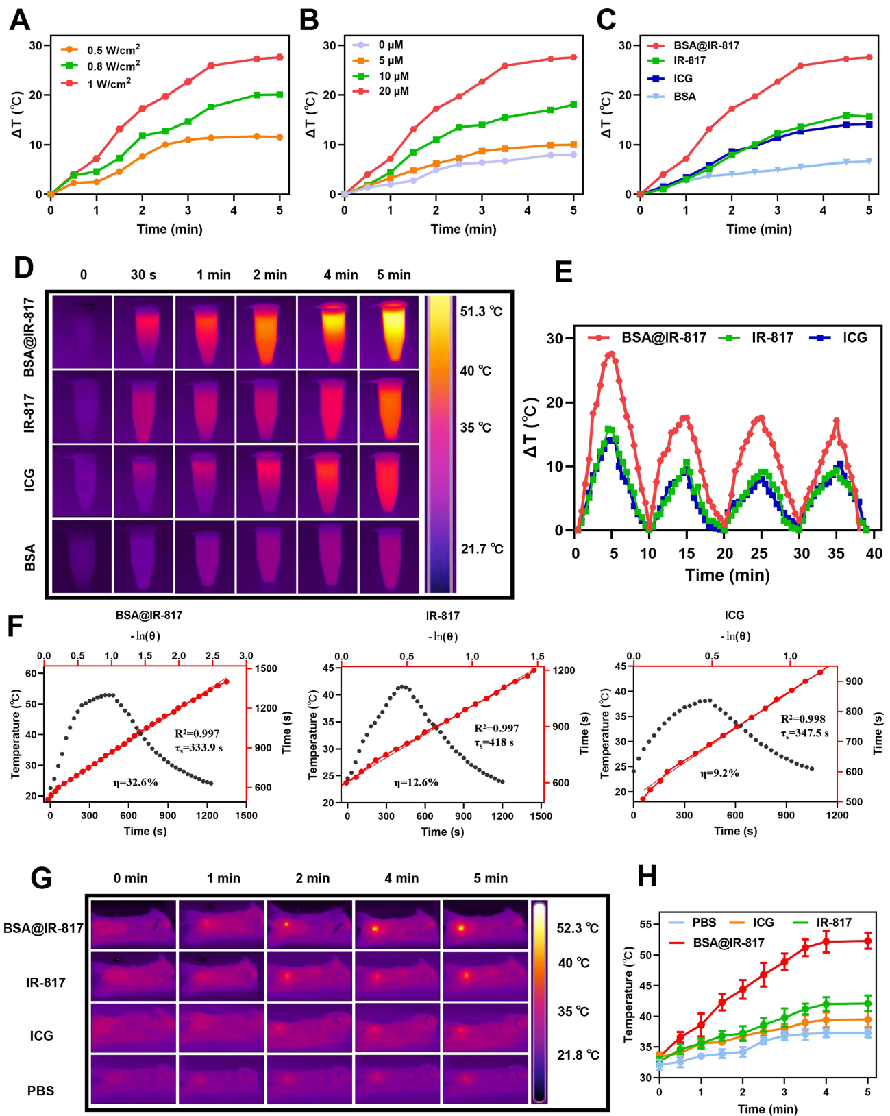
Figure 4 Evaluations BSA@IR-817 photothermal properties. (A) Temperature increase of BSA@IR-817 (20 \mu\text{M} ) in PBS under an 808 nm laser with different exposure intensities (0.5, 0.8, 1 \text{W}/\text{cm}^2 ). (B) Temperature increase of BSA@IR-817 at different concentrations (0, 5, 10, and 20 \mu\text{M} ) under an 808 nm laser (1 \text{W}/\text{cm}^2 ). (C) Temperature change of BSA@IR-817, IR-817, ICG and BSA (20 \mu\text{M} ) upon exposure to 808 nm laser (1 \text{W}/\text{cm}^2 ) for different intervals. (D) Infrared thermal images of (C) . (E) Temperature changes of BSA@IR-817, IR-817 and ICG during four circles of heating-cooling processes (1 \text{W}/\text{cm}^2 , 5 min). (F) Photothermal conversion efficiency (PCE) of BSA@IR-817, IR-817 and ICG (20 \mu\text{M} , 1 \text{W}/\text{cm}^2 ). (G) Infrared thermographic images of the B16-F10 cell tumor-bearing mice after irradiation (1 \text{W}/\text{cm}^2 , 5 min). (H) Change in tumor temperature as a function of the irradiation time.
