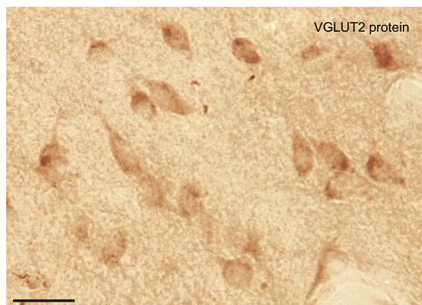
Figure 9 VGLUT2 protein expression in the pulvinar is largely confined to cell bodies and processes instead of terminals. Scale bar is 25 \mu\text{m} .
