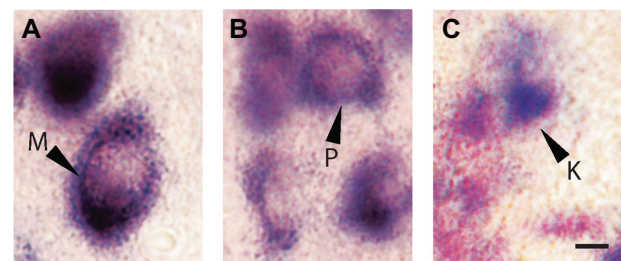
Figure 5 LGN cell types can be differentiated according to pattern of staining for VGLUT2 mRNA. A ) M cells are large and exhibit strong nuclear staining for VGLUT2 mRNA. B ) P cells are slightly smaller but also show intense staining for VGLUT2 . C ) K cells are the smallest of all three and show weak, diffuse staining for VGLUT2 . Scale bar is 50 \mu m.
