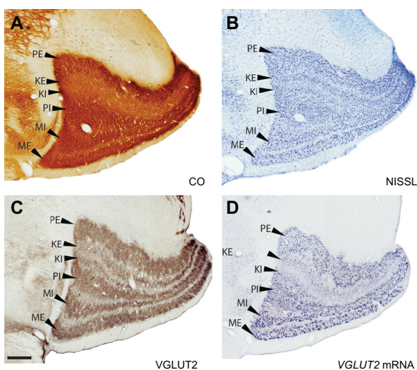
Figure 2 Serial sections through part of the rostral lateral geniculate nucleus (LGN) stained for (A) cytochrome oxidase (CO), (B) Nissl, (C) VGLUT2 protein and (D) VGLUT2 mRNA. Scale bar is 0.5 mm. Coronal sections, lateral is right.
