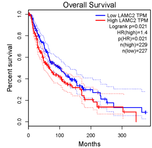
LAMC2
