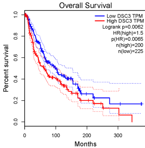
DSC3
